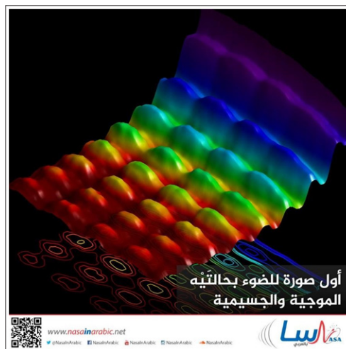
Figure 2: The first image of light in its wave and particle states.
