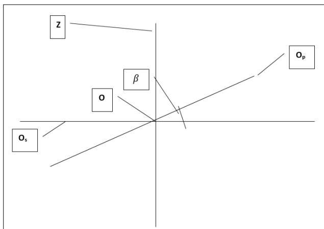
Picture 1: Cross section of the solar system
