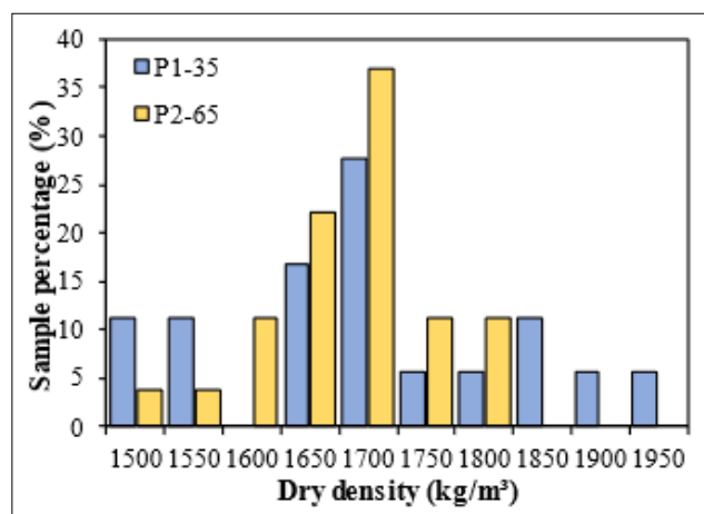
Figure 8: Dry Density of Platinum Tailings from 65 mm MOSTAP Sampler
