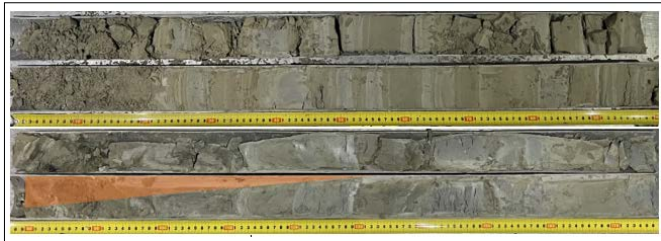
Figure 3: MOSTAP Samples Taken from above (top) and below (bottom) the Phreatic Surface
