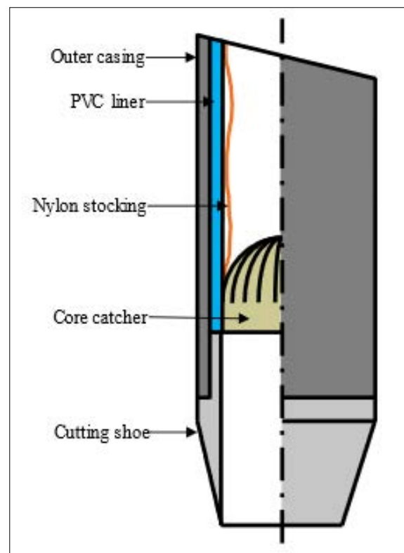
Figure 1: Schematic section of a MOSTAP soil sampler
