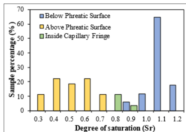
Figure 9: Degree of Saturation Calculated from MOSTAP Samples
