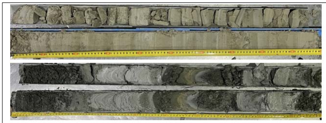
Figure 2: MOSTAP samples from P2-65 after opening showing smearing of clayey samples
