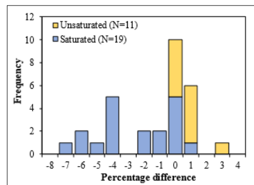
Figure 5: Mass Differences between Post-Extraction and Laboratory Measurements
