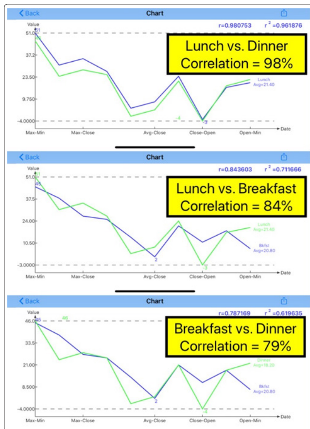
Figure 7: Correlation study among 3 meal character differences
