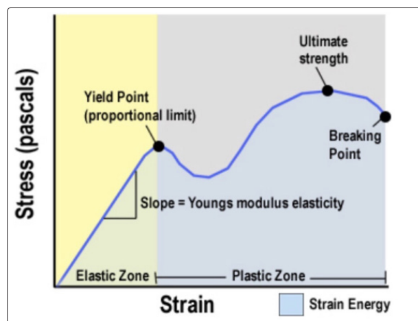
Figure 1: Stress-Strain-Young's modulus, Elastic Zone vs. Plastic Zone
