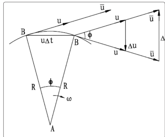
Figure 2: On body B the \frac{du}{dt} and \frac{d\bar{u}}{dt} coexistence [4]
