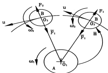
Figure 4: A expansion model of the Universe
