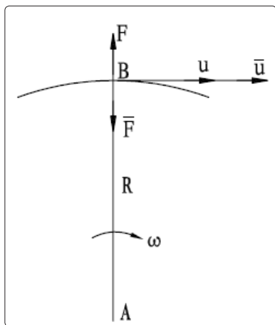
Figure 3: On body B the F and \bar{F} coexistence and the new Universe model
