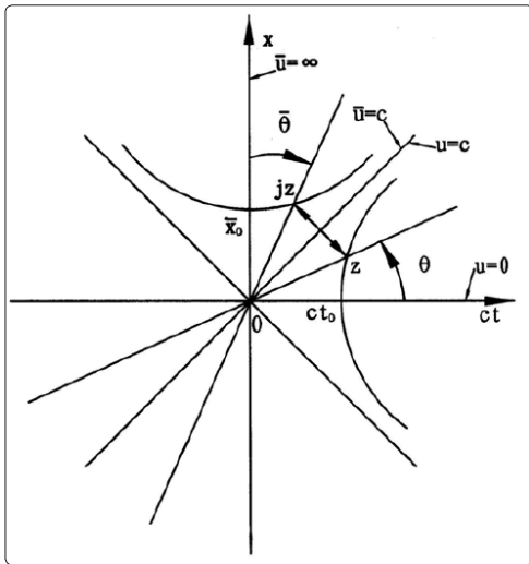
Figure 1: Mathematical theory of space-time with SASC and ILS
