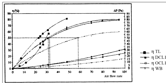
Figure 6: Evolution of thermal efficiency (where I_{GS} = 1063.5\text{W/m}^2 ) and charge losses in relation to air flow as concerns WB solar panels and those provided with different types of baffles (i.e. DCL1, OCL1 and then TL), as at the Valenciennes site
