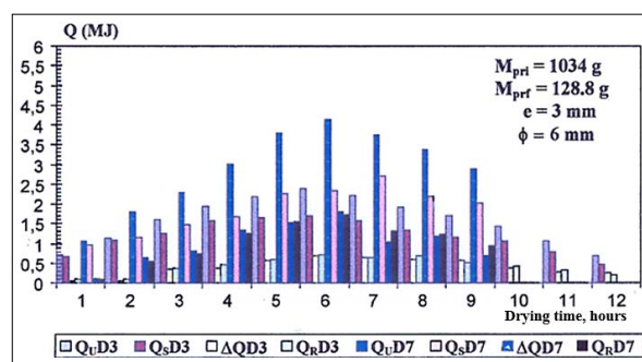
Figure 12: Variations in quantities of heat ( Q ) in relation to drying time with flows of 31.3\text{m}^3/\text{h.m}^2 and 70\text{m}^3/\text{h.m}^2 using an WB type solar panel (without baffles)
