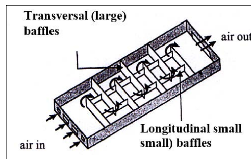
Figure 7: Solar panel equipped with TL type baffles
