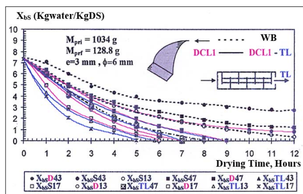
Figure 8: Evolution of the water content ( X_{bs} ) in relation to drying time measured at the first and fourth trays with flows of 31.3m 3 /h.m 2 and 70m 3 /h.m 2 using WB, DCL1 and TL type solar panels, data recorded on a typical July day at the Valenciennes site.
