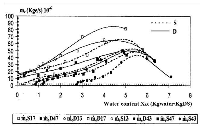
Figure 11: Evolution of the drying speed ( m_e ) in relation to water content to the point when the product is completely dried with flows of 31.3\text{m}^3/\text{h.m}^2 and 70\text{m}^3/\text{h.m}^2 using WB and DCL1 type solar panels
