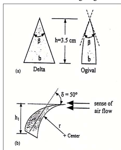
Figure 5: Delta and Ogival Baffles (a) Before Bending; (b) After Bending
