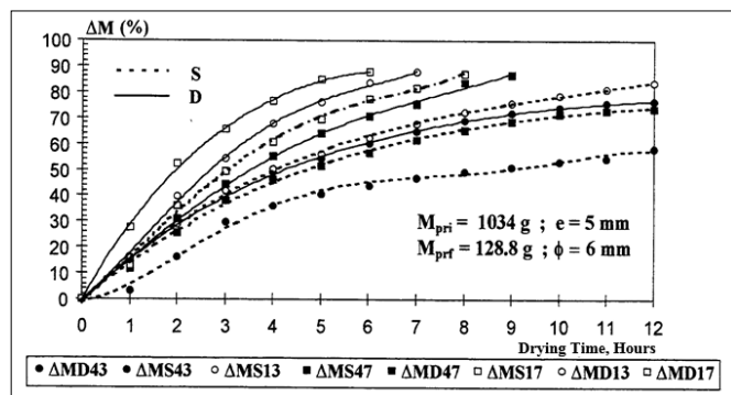
Figure 9: Evolution of the loss of mass ( \Delta M ) of plums in relation to drying time measured at the first and fourth trays with flows of 31.3\text{m}^3/\text{h.m}^2 and 70\text{m}^3/\text{h.m}^2 using DCL1 and TL type solar panels, data recorded on a typical July day at the Valenciennes site
