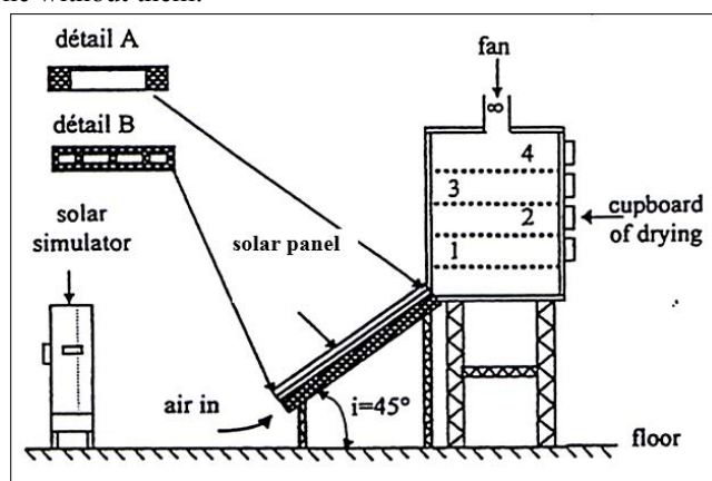
Figure 1: Experimental device
