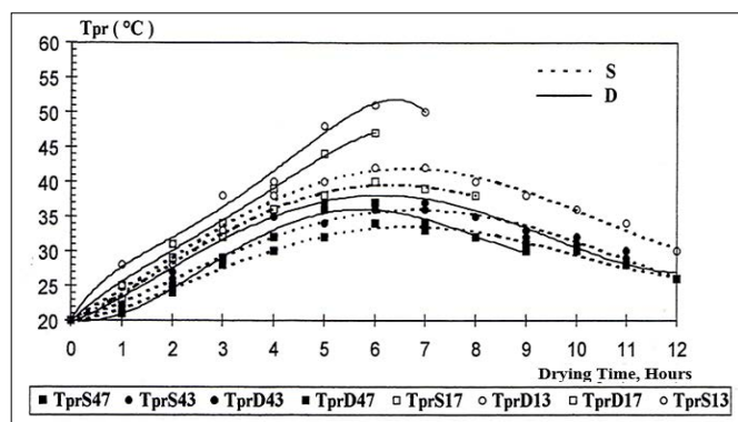
Figure 10: Evolution of the temperature of Lemon in relation to drying time measured at the first and fourth trays with flows of 31.3\text{m}^3/\text{h.m}^2 and 70\text{m}^3/\text{h.m}^2 using WB, DCL1 and TL type solar panels
