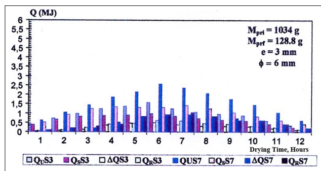
Figure 13: Variations in quantities of heat (Q) in relation to drying time with flows of 31.3m 3 /h.m 2 and 70m 3 /h.m 2 using a solar panel equipped with DCL1 baffles
