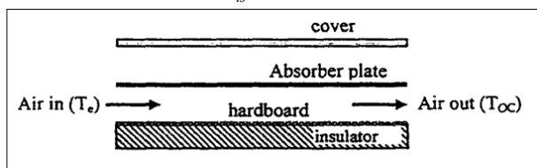
Figure 2: Solar Air Flat Plate Collector without Obstacles
