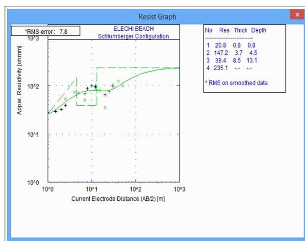
Figure 4: Elechi Beach VES curve and Model
