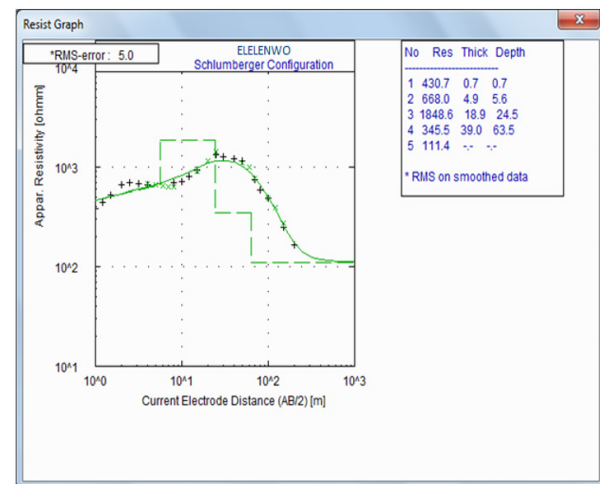
Figure 10: Elenwo VES curve and Model
