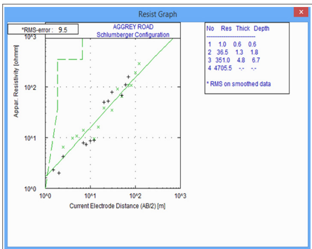
Figure 7: Aggrey Road VES curve and Model
