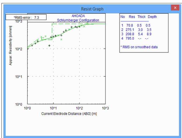
Figure 6: Ahoada West VES curve and Model
