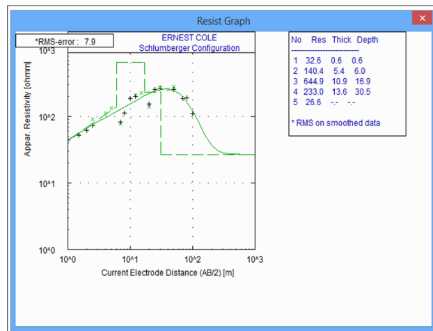
Figure 2: Ernest Cole VES curve and Model
