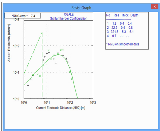
Figure 5: Ogale Eleme VES curve and Model
