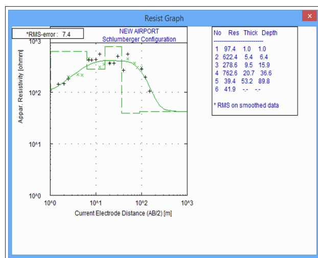
Figure 3: New Airport VES curve and Model
