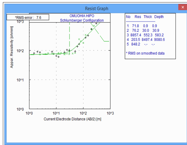
Figure 8: Ipo 3 VES curve and Model
