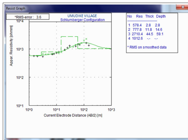
Figure 9: Umuodike VES curve and Model
