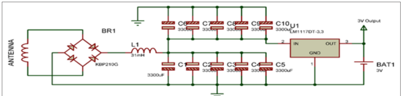
Figure 2: UHF RFID Power Supply Unit
