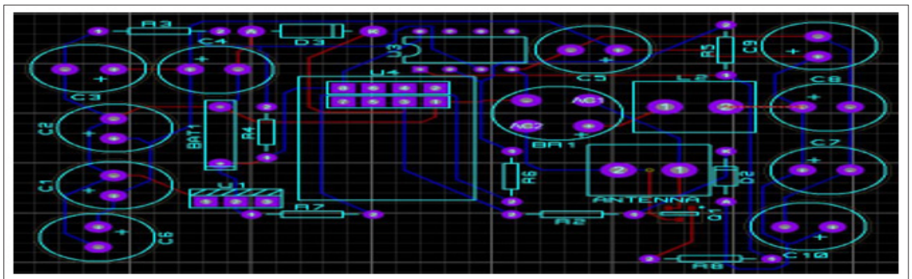
Figure 7: PCB Complete Circuit Diagram of UHF RFID Tag
