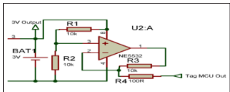
Figure 4: UHF Tag Signal Amplifier Circuit
