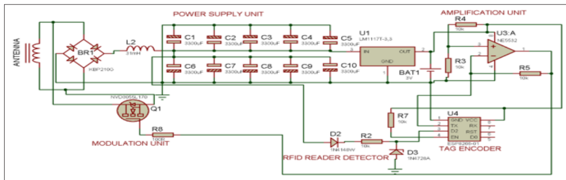
Figure 6: Complete Circuit Diagram of UHF RFID Tag
