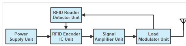
Figure 1: Active/Passive RFID Tag Block Diagram
