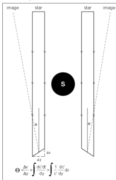
Figure 1: Schematic diagram showing light rays emitted by stars to follow straight-line trajectories as they pass near the sun. Because of gravitational effects the speed of the light rays c' is known to increase with gravitational potential, with the effect that the corresponding Huygens wave front gradually rotates away from the sun. As discussed in the text, the normal to a given wave front points out the direction from which the light appears to have come, causing the star images to be displaced by an angle \Theta during solar eclipses.
